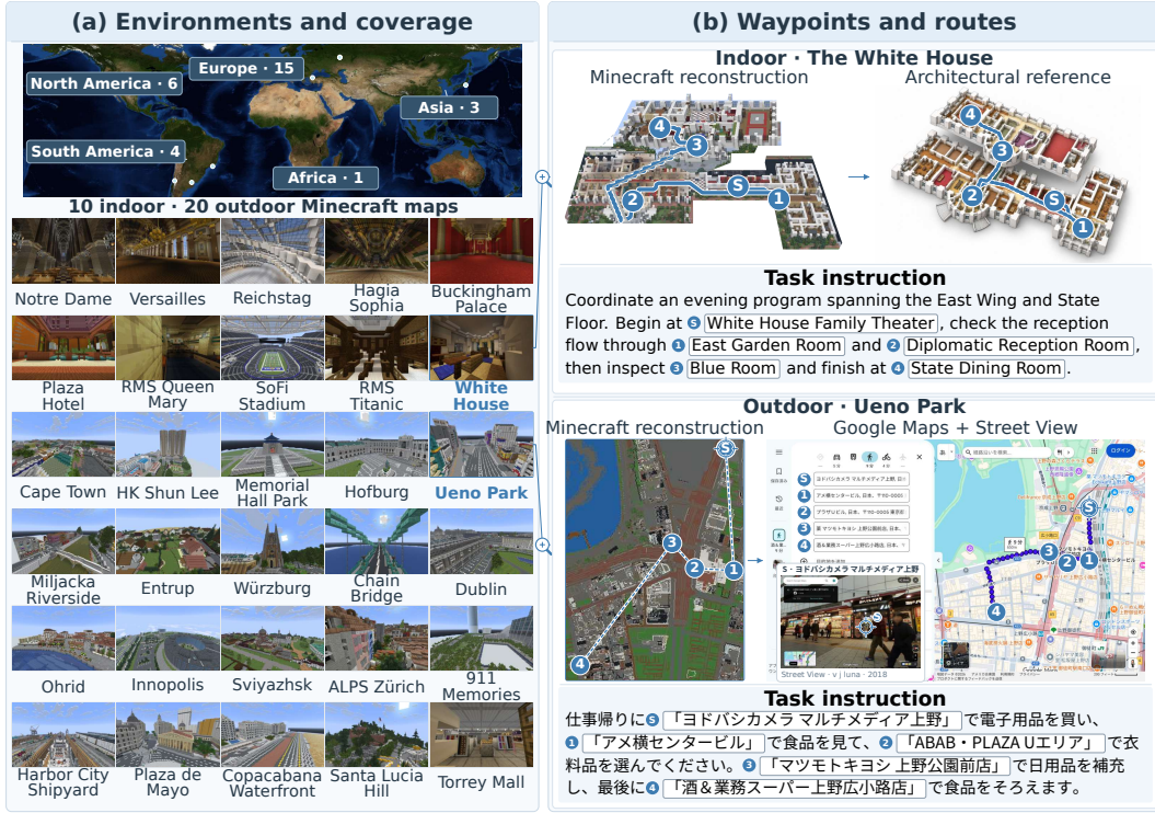
Figure 1: Overview of MINE ODYSSEY environments and task construction. (a) 30 Minecraft reconstructions and geographic coverage. (b) Task construction with White House and Ueno Park examples: reference locations are mapped to waypoints and ordered into navigation tasks. S denotes the start; numbered markers and dashed lines indicate visit order.
